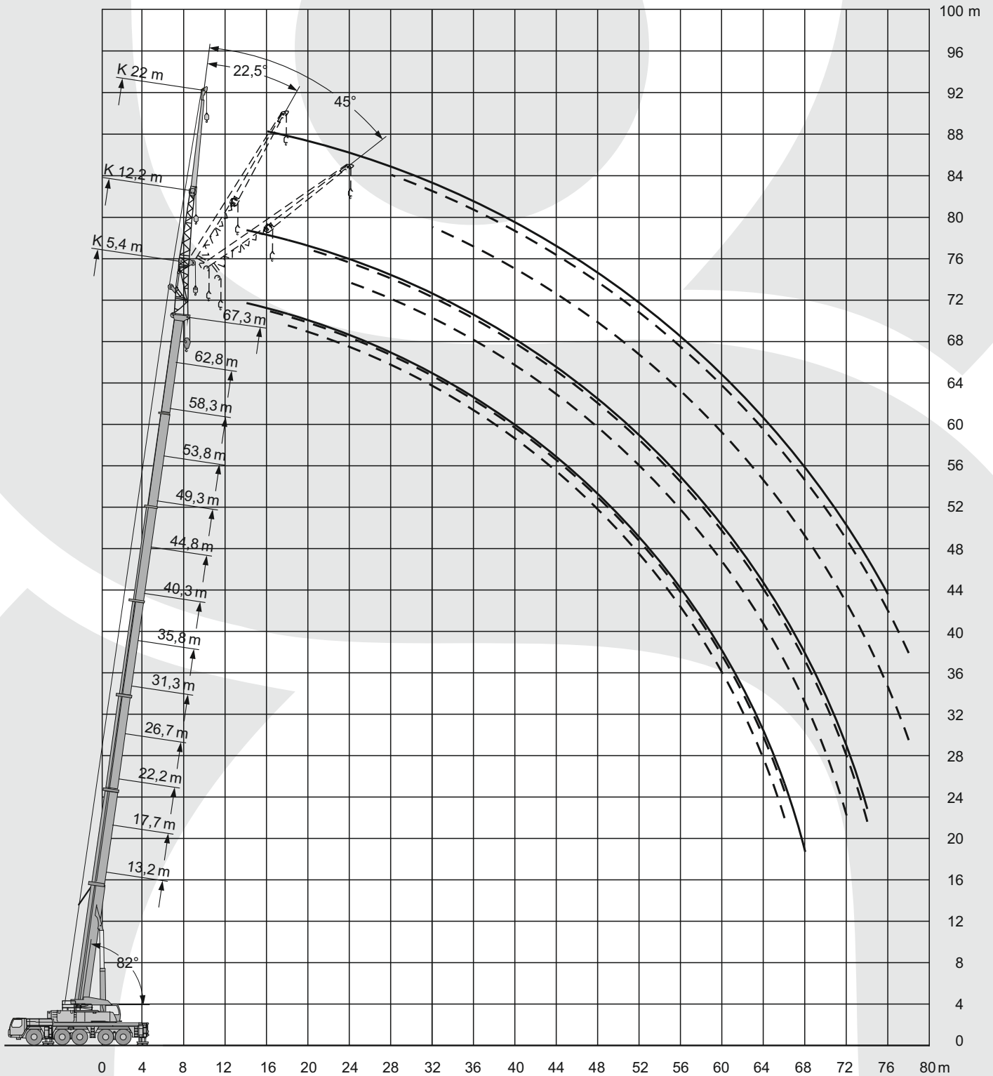
Working range: main boom + fix jib
